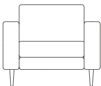
ARMCHAIR WIDTH 860 DEPTH 770 OVERALL HEIGHT 700 SEAT HEIGHT 430
