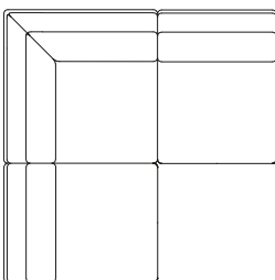
3 SEAT 90° CORNER UNIT WIDTH 1370 DEPTH 1370 OVERALL HEIGHT 700 SEAT HEIGHT 430
