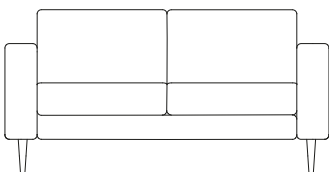
2 SEAT SOFA WIDTH 1460 DEPTH 770 OVERALL HEIGHT 700 SEAT HEIGHT 430
