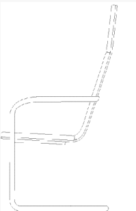
HIGH BACK CANTILEVER CHAIR WIDTH 560 DEPTH 680 BACK HEIGHT 1140 SEAT HEIGHT 460 ARM HEIGHT 660
