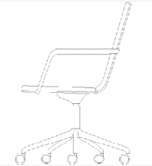
MEDIUM BACK 5 STAR SWIVEL CHAIR WIDTH 560 DEPTH 680 BACK HEIGHT 915 SEAT HEIGHT 460 ARM HEIGHT 670
