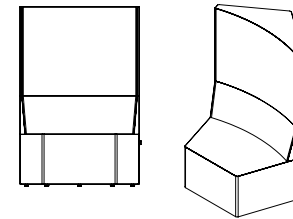
Seat Module - High Back Height 1410 Width 935 Depth 890 Seat Height 410
