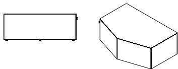
Long Seat Module - No Back Height 410 Width 1120 Depth 770 Seat Height 410
