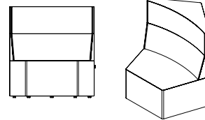
Seat Module - Medium Back Height 1010 Width 935 Depth 890 Seat Height 410
