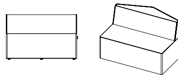
Long Seat Module - Low Back Height 710 Width 1120 Depth 770 Seat Height 410
