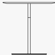
DB/75RD/74H WIDTH 750 HEIGHT 740
