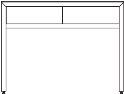
1000 x 400 x 750 Slab ended base with adjustable levellers
